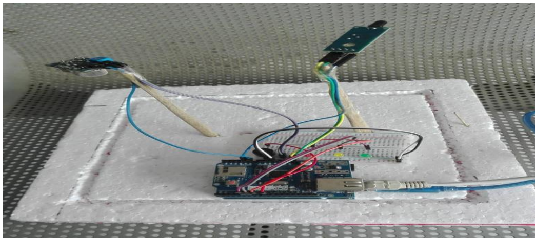
Figure 3 Prototype of fire hazard detection using Arduino
