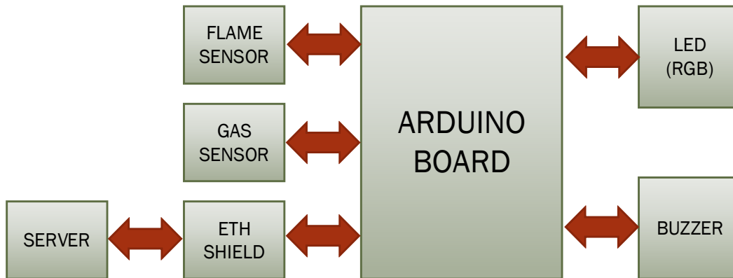
Figure 2 The architecture of fire hazard system
